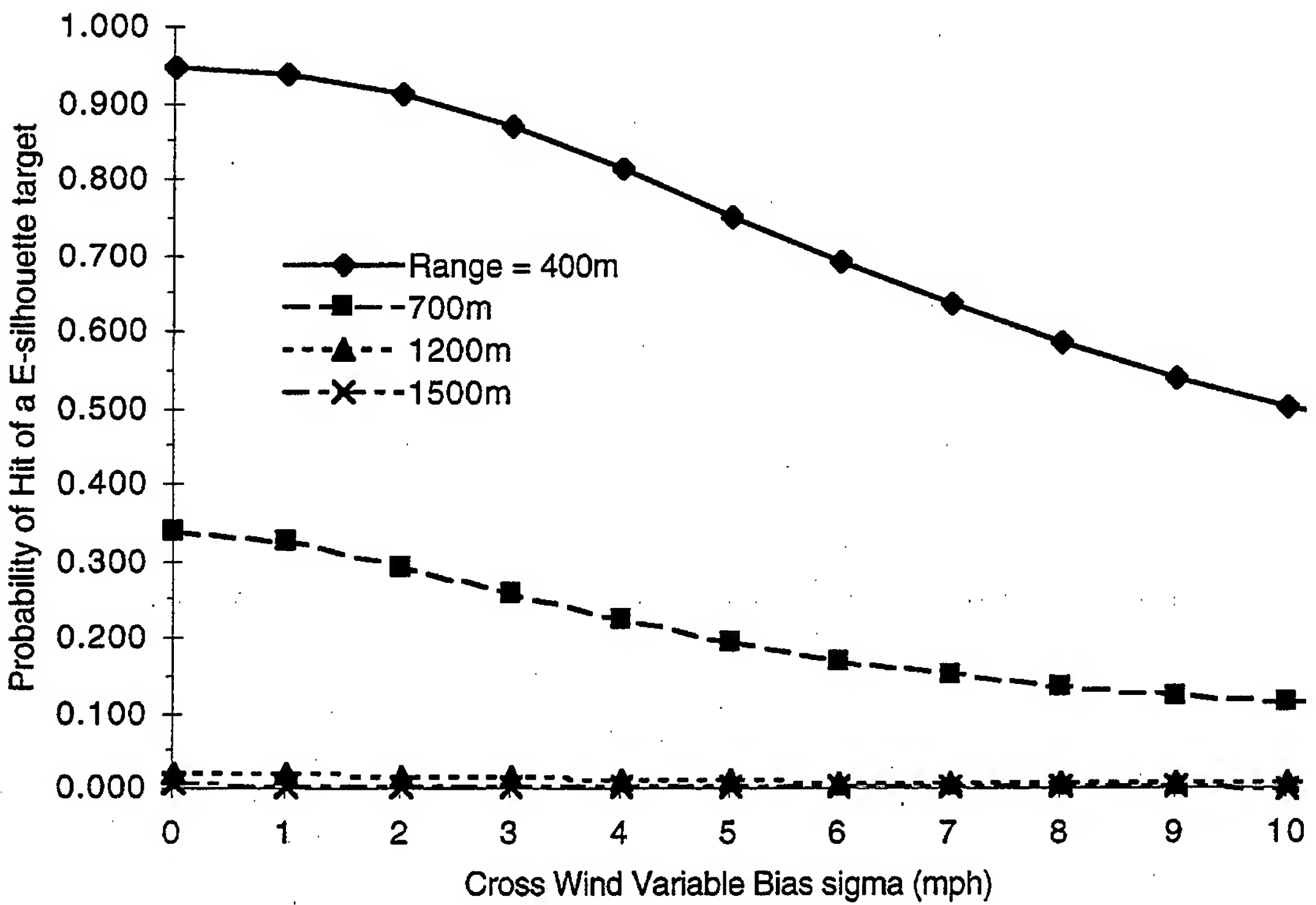
Figure 11. Error Budget Sensitivity, Crosswind Variable Bias.
